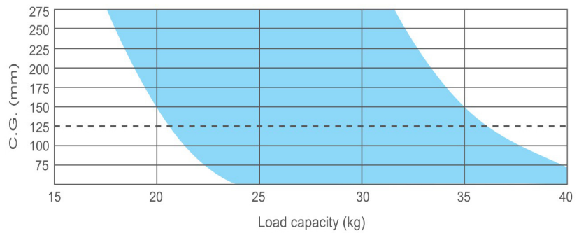
CHX Counterbalance chart
